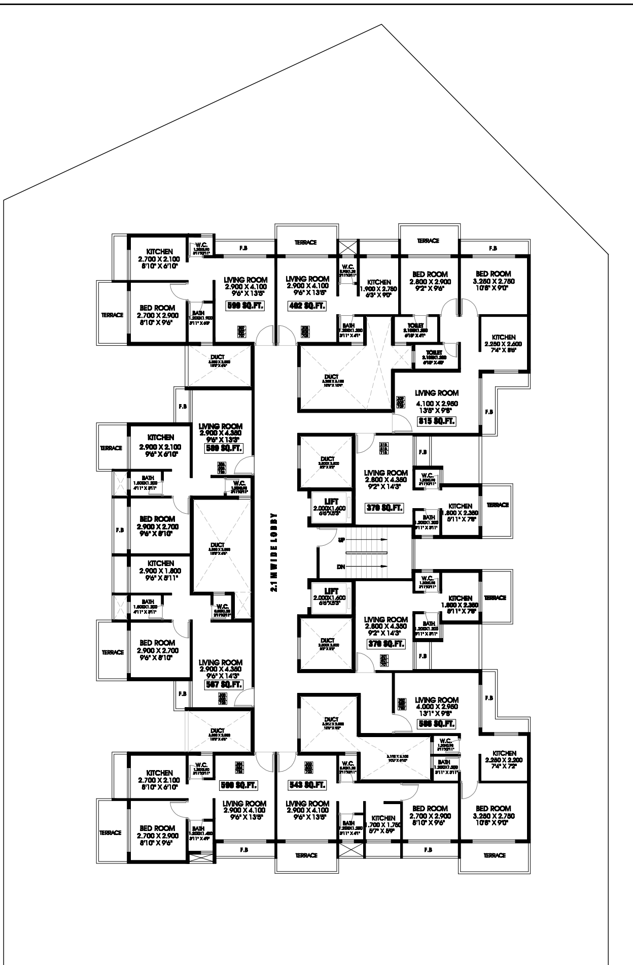
← 15 M . WIDE ROAD → TYPICAL FLOOR PLAN ( 3RD, 5TH & 7TH )
